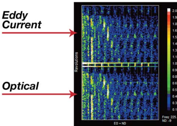
Figure 2: Results from tip-timing trials of the T 3 on a Spey RB168-101 engine at QinetiQ's open air engine test facility, Shoeburyness, UK. The T 3 produced comparable results to optical sensors even at high frequency, but was unaffected by the rain which contaminated the optical sensors.
